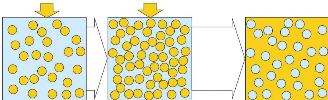
Figure 2: When making mayonnaise, oil is added to water. If too much oil is added at once, the mayonnaise turns from an oil in water emulsion to a water in oil emulsion.
