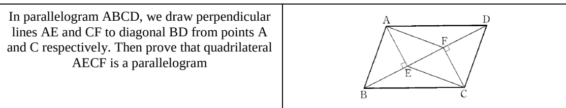
Fig. 3: Proof problem about parallelogram (Okamoto et al, 2012, p. 133)
