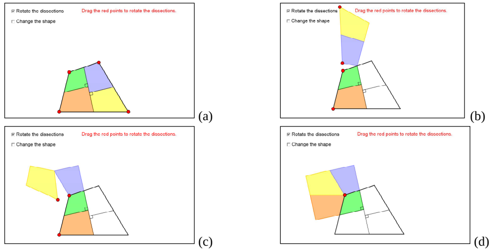
Figure 3: The GeoGebra task of dissecting a quadrilateral into a rectangle
