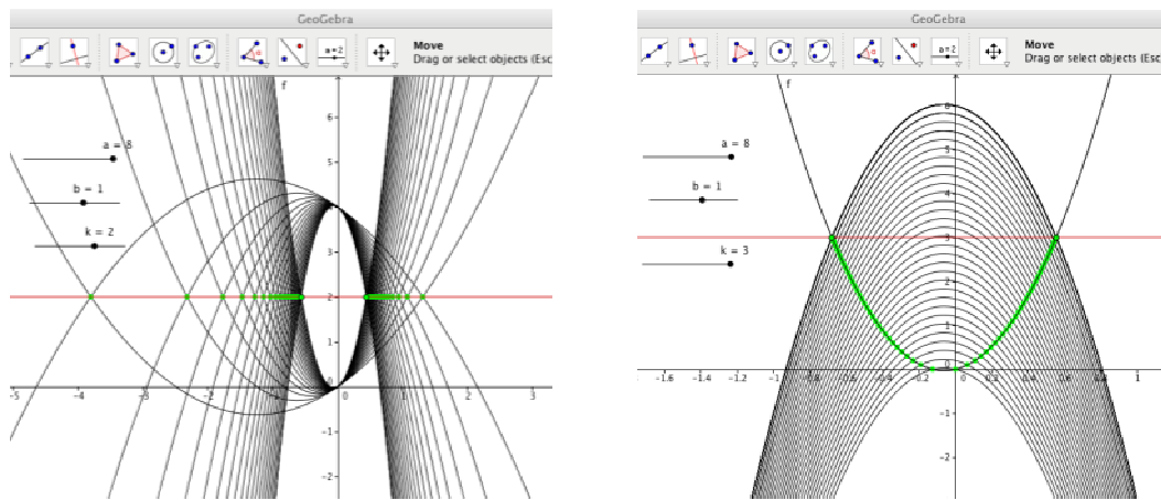
Figure 3. Dynamic reflection of graphs in the line y = k using GeoGebra.
