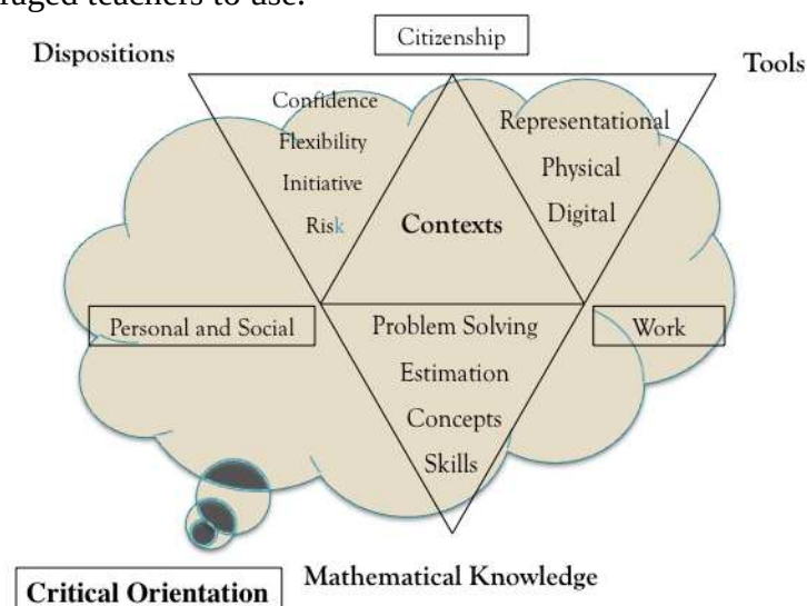
Figure 1. Numeracy model
