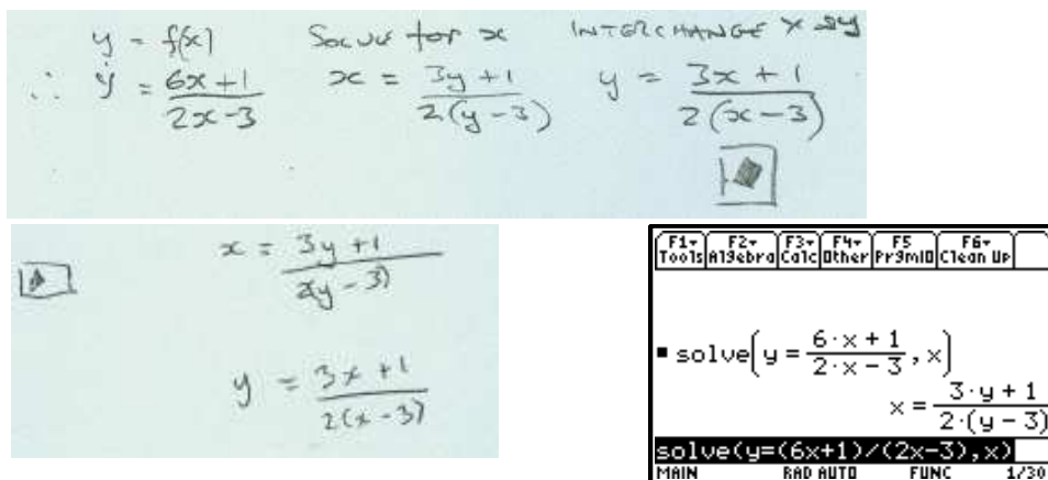
Figure 1. Integration of CAS in the task:
