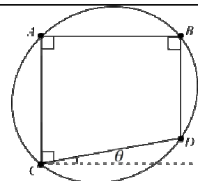
Author-generated diagram of Penny and Carol's solution
