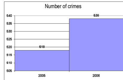
Figure 3: Task "crimes"
